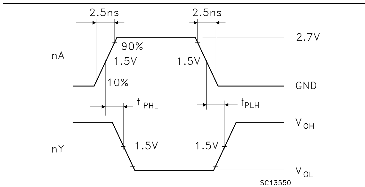
WAVEFORM : PROPAGATION DELAY ( f=1\text{MHz} ; 50% duty cycle)
